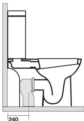
curva tecnica art. 900102 waste pipe art. 900102
