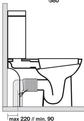
curva tecnica variabile 90° art. 900104 variable waste pipe 90° art. 900104
