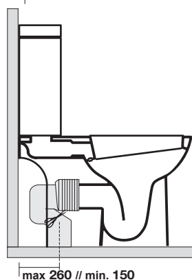
curva tecnica variabile art. 7619 variable waste pipe art. 7619
